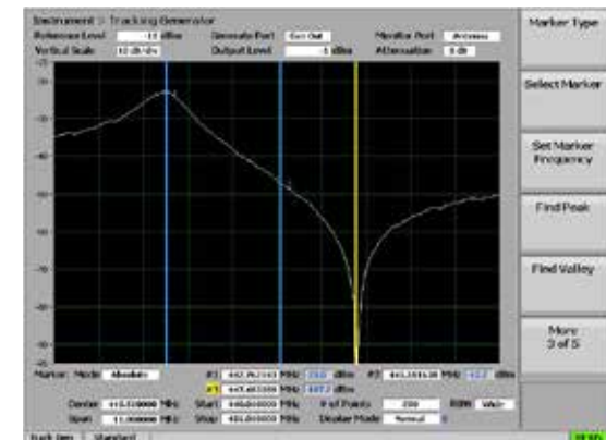
Tracking Generator
